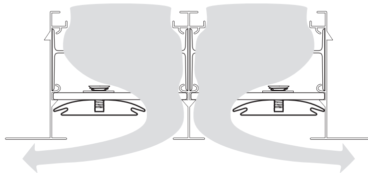
HORIZONTAL DISCHARGE 2 WAYS
