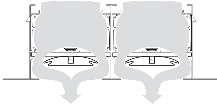
VERTICAL DISCHARGE
